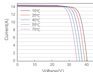
Current-Voltage Curve JAM54D40-440/LB/1500V
