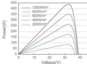
Power-Voltage Curve JAM54D40-440/LB/1500V
